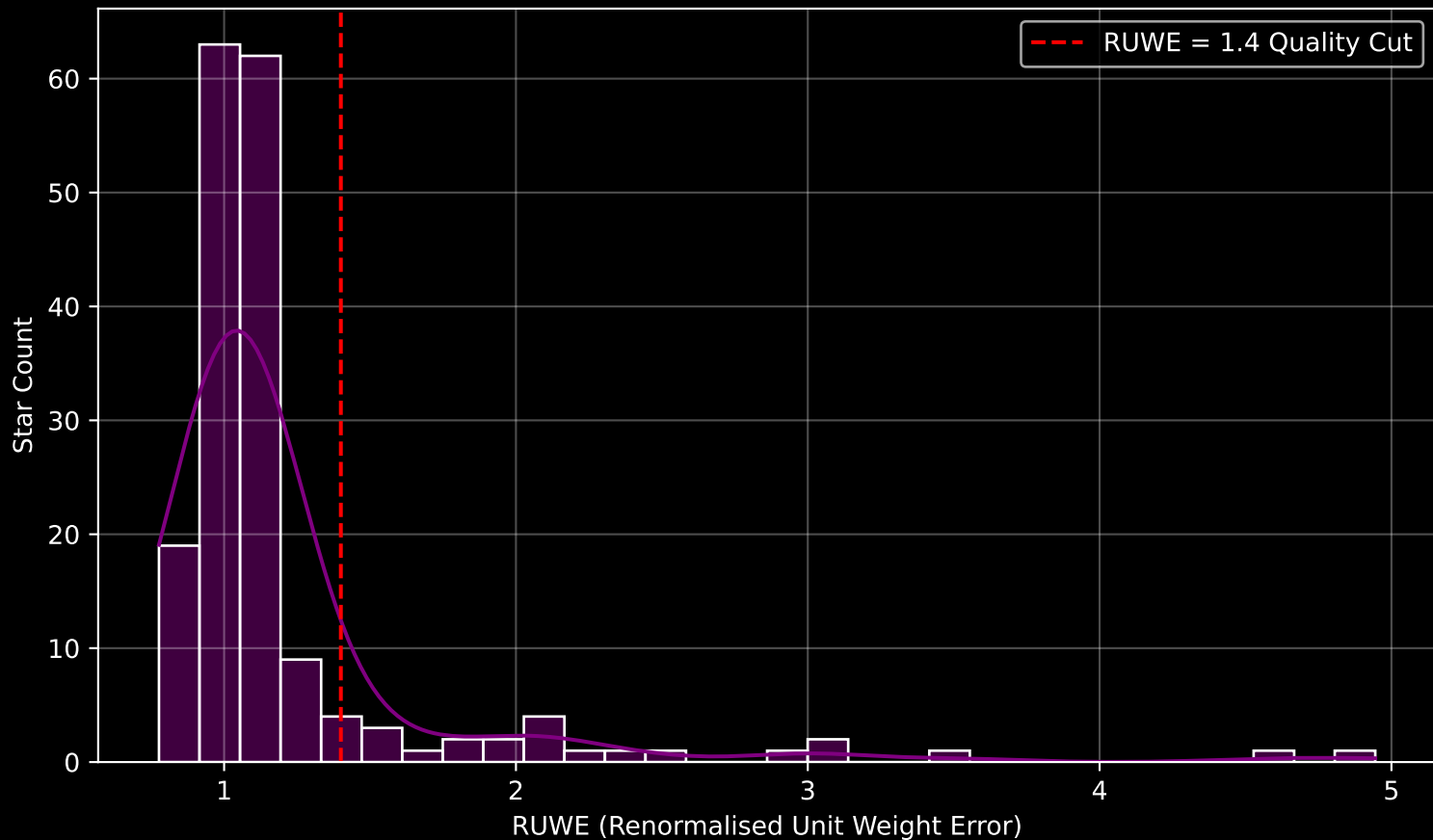
GAPOGEE DR17 Field [193+23_MGA] RUWE Distribution (n= 178)
