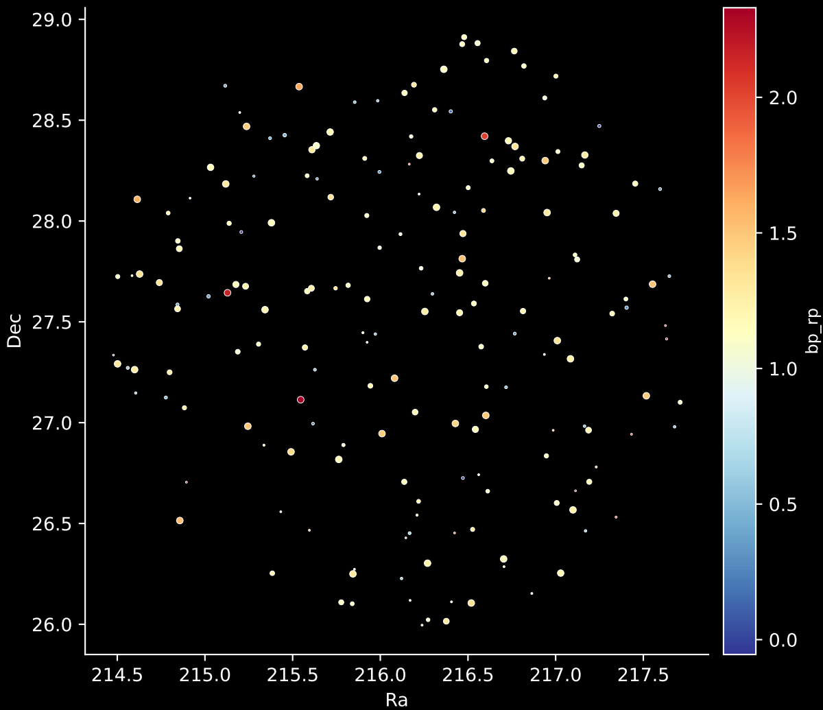
APOGEE DR17 Field: [193+23_MGA] Stars: 184
