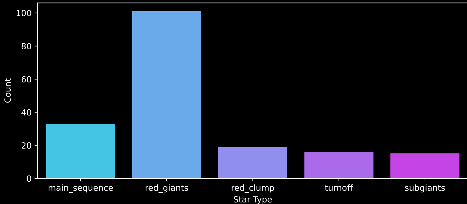
APOGEE DR17 Field: [193+23_MGA] Count plot of Star Type
