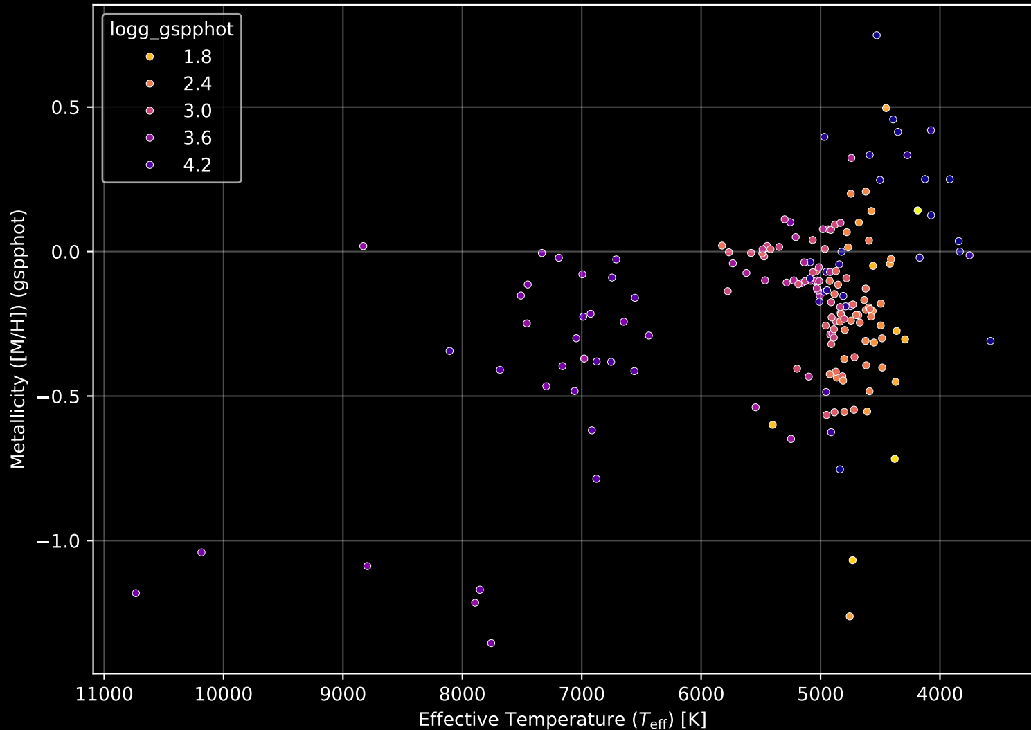
APOGEE DR17 Field: [193+23_MGA] Stellar Population Parameters (n= 184)
