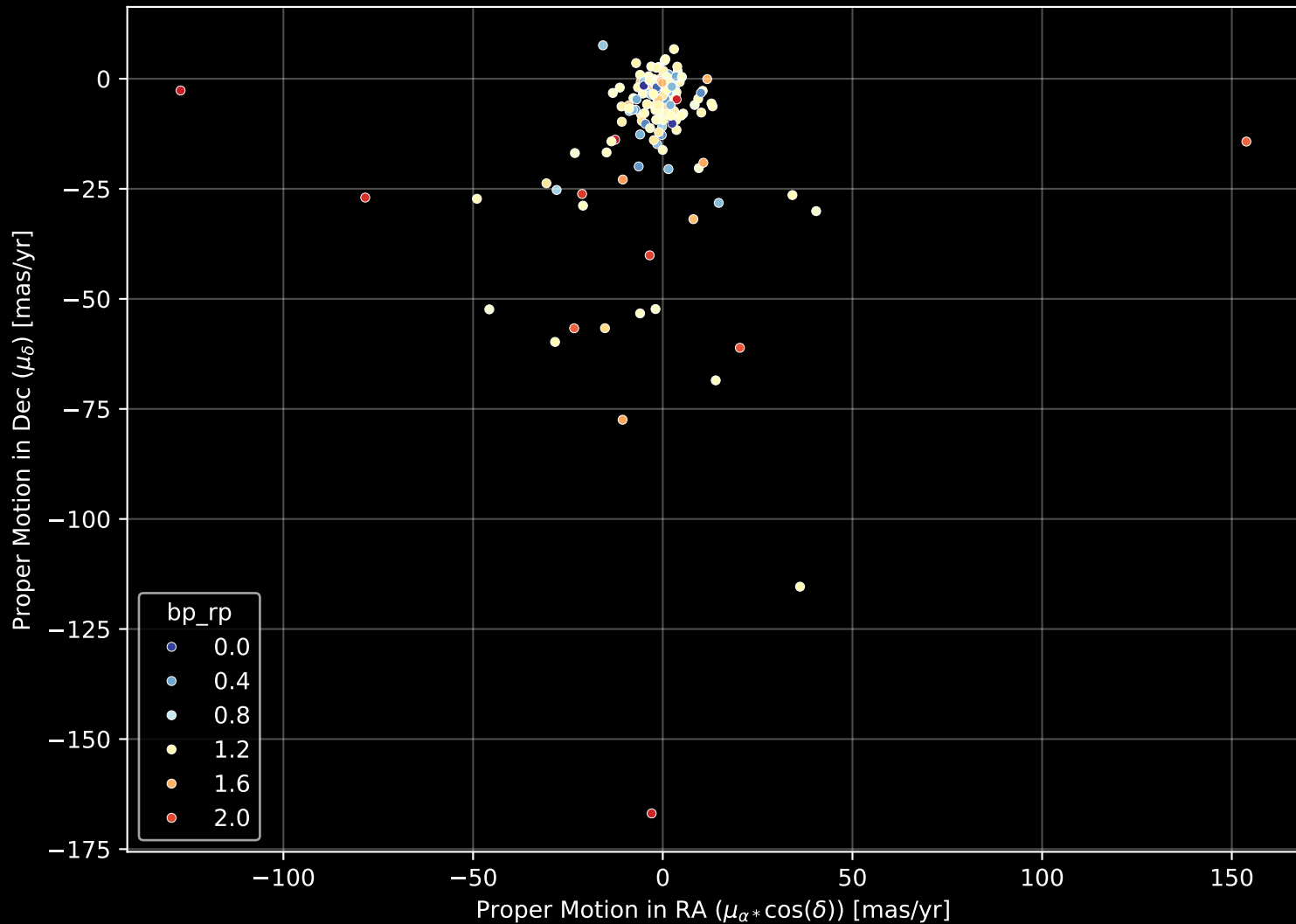
APOGEE DR17 Field: [193+23_MGA] Proper Motion Diagram (n= 184)
