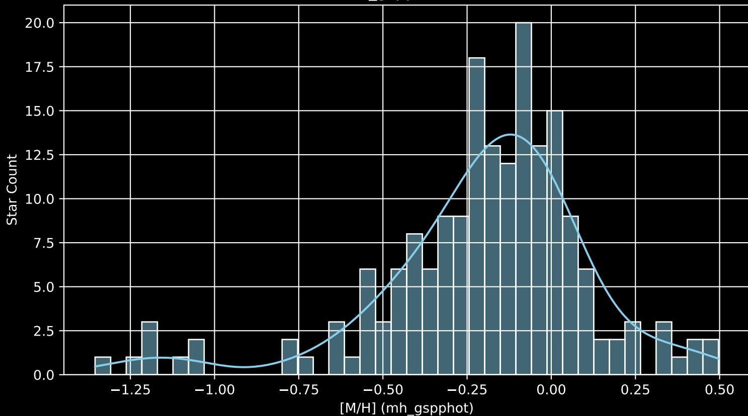
APOGEE DR17 Field: [193+23_MGA [M/H] (mh_gspphot) (n= 183)
