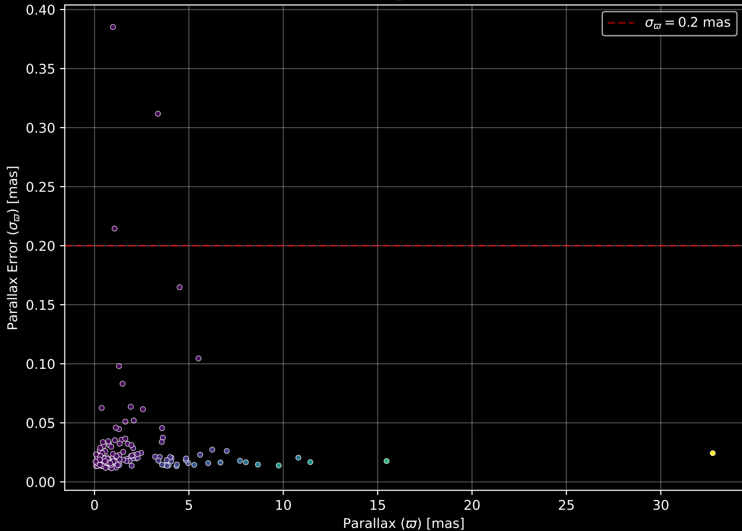
APOGEE DR17 Field: [193+23_MGA] Parallax Quality (n= 184)
